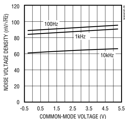
NOISE VOLTAGE DENSITY vs. COMMON-MODE VOLTAGE
